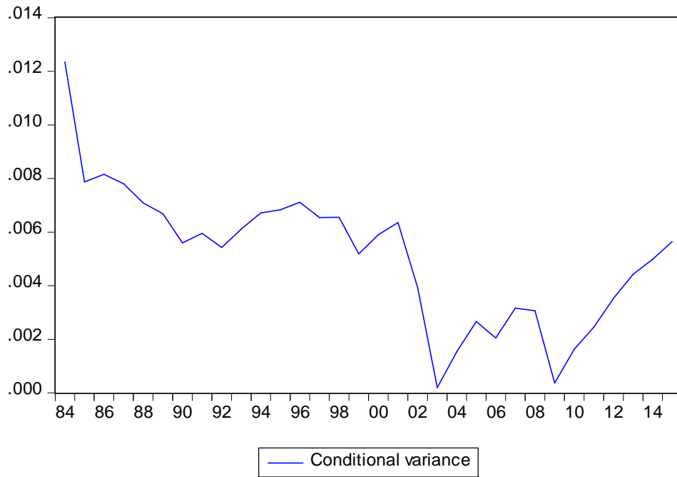
Graph 2: Conditional Variance derived from GARCH estimation based on Equation 1
